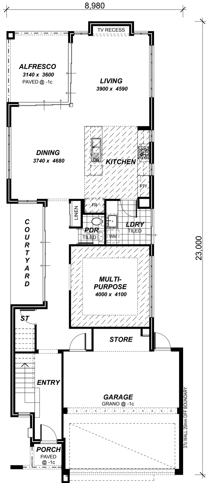
LOWER FLOOR PLAN
